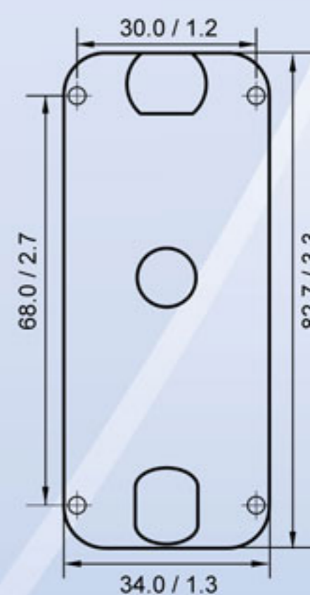
Mifare access control module board
